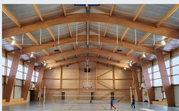
GYMNASE DIAMANT® Gonneville-la-Mallet (76)
